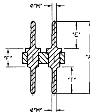
SECTION B-B SCALE 4:1
