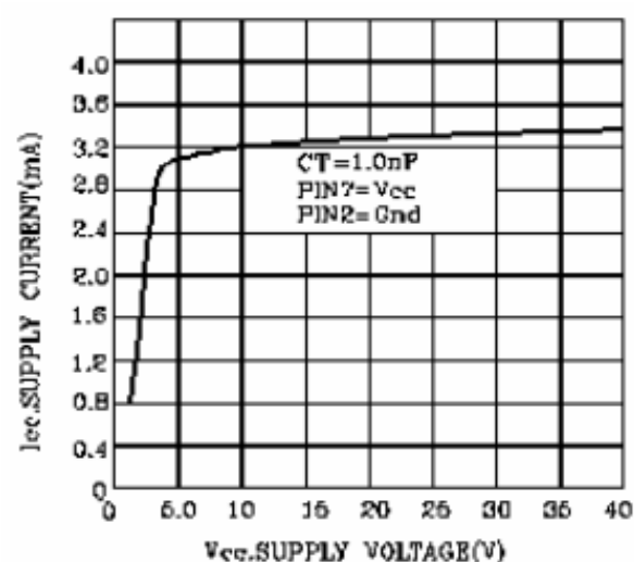
FIGURE 6.STANDBY SUPPLY CURRENT versus SUPPLY VOLTAGE
