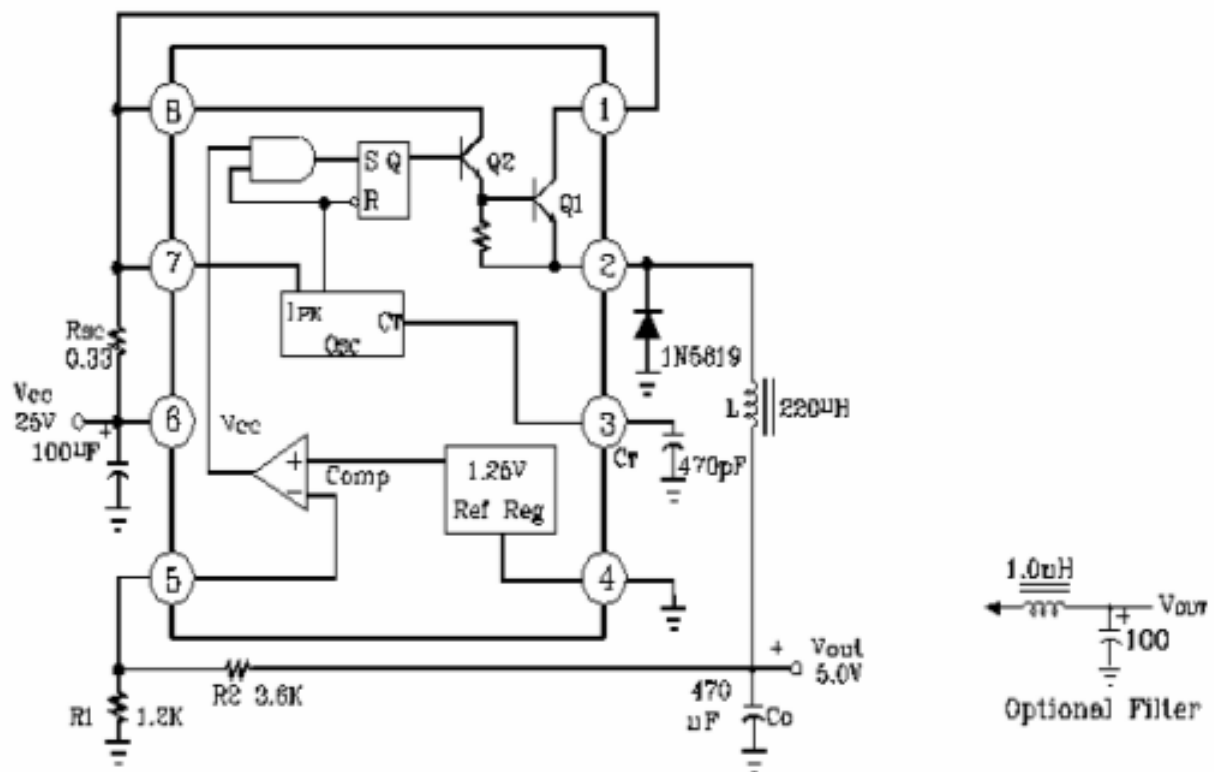
FIGURE 3.STEP-DOWN CONVERTER
