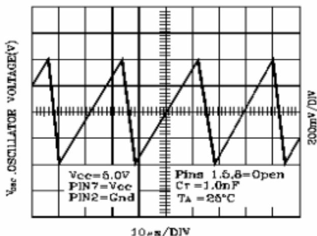
FIGURE 2.TIMING CAPACITOR WAVEFORM
