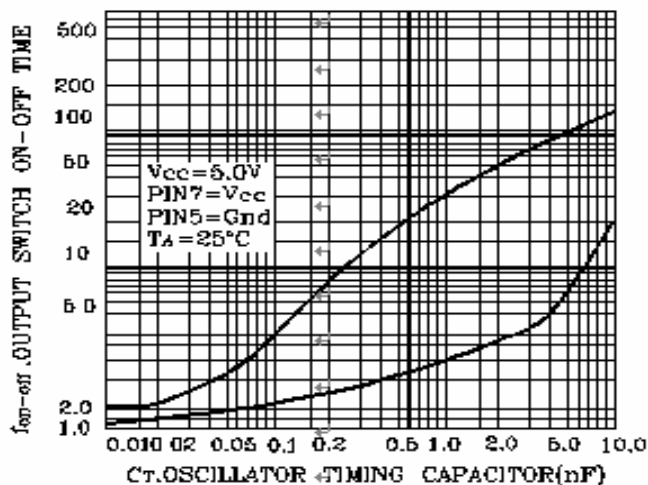
FIGURE 1.OUTPUT SWITCH ON-OFF TIME versus OSCILLATOR TIMING CAPACITOR
