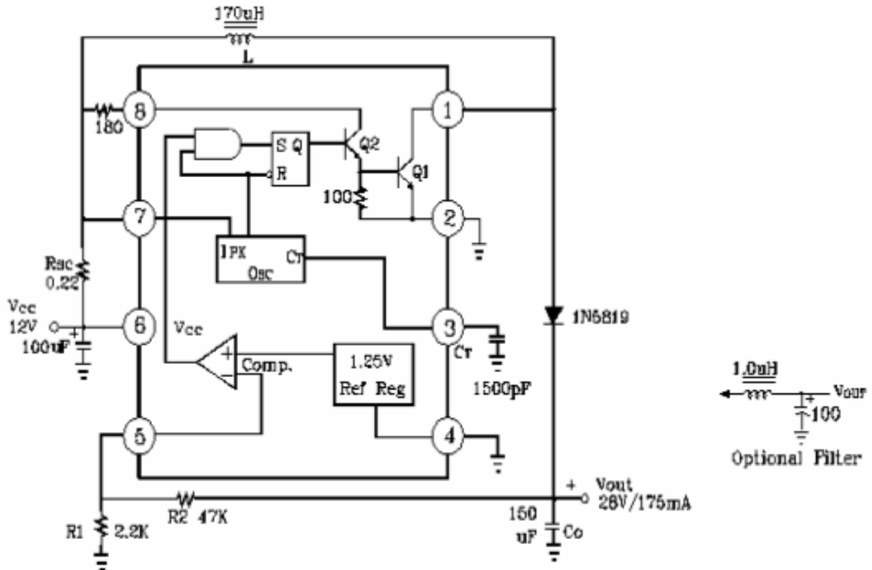
FIGURE 1.STEP-UP CONVERTER
