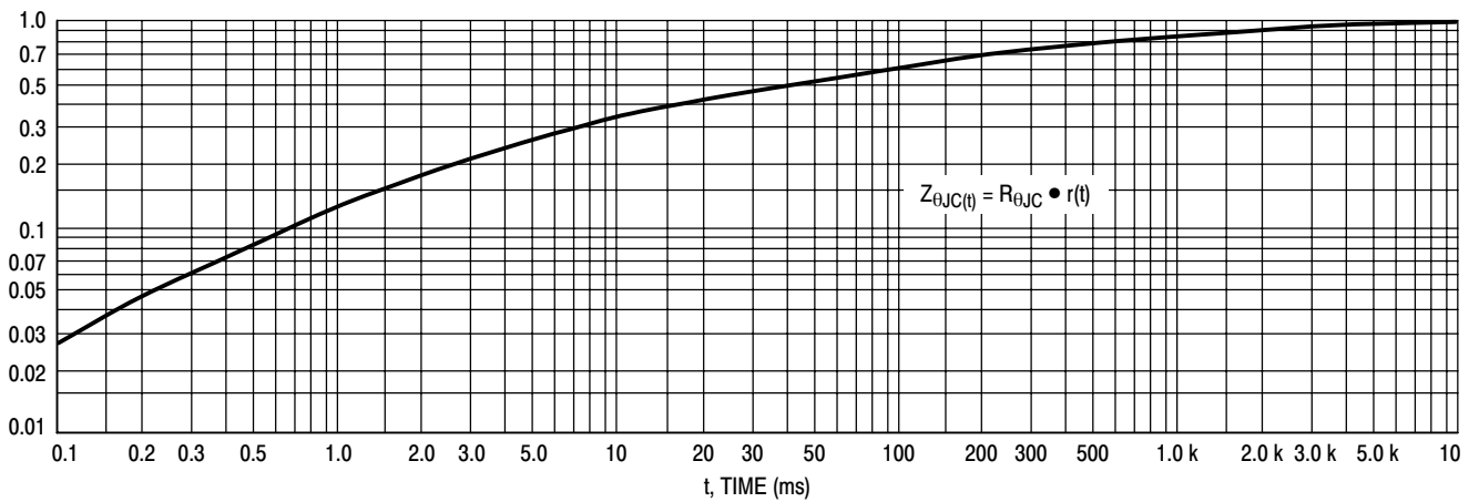
Figure 5. Thermal Response
