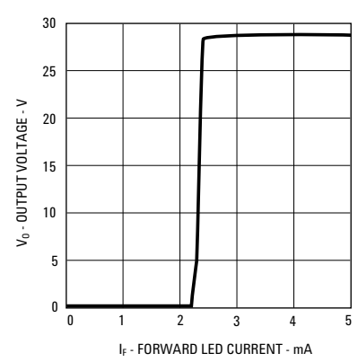
Figure 15. Transfer Characteristics
