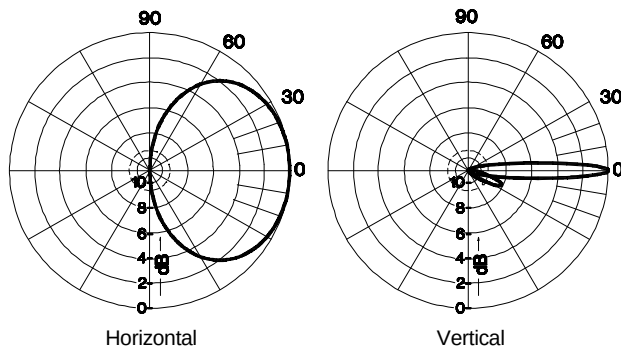
Antenna Patterns
