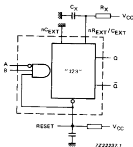
Fig. 11 Power-up output pulse elimination circuit.
