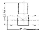
BNC Tee Adapter, J/J/J
