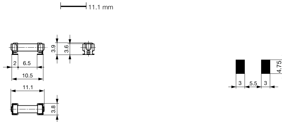
Soldering pads
