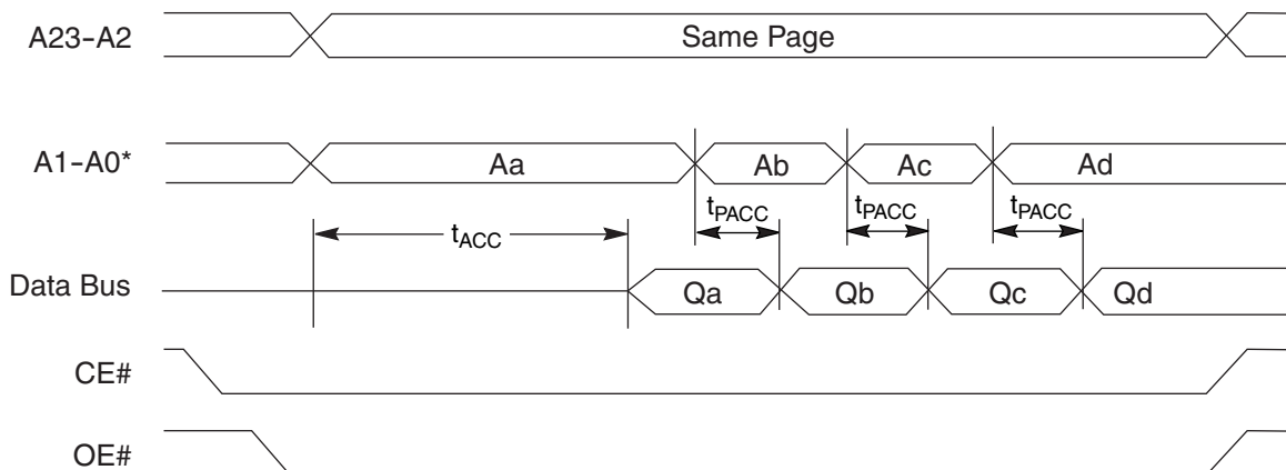
Figure I3. Read Operation Timings
