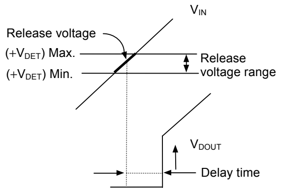
Figure 30 Release Voltage
