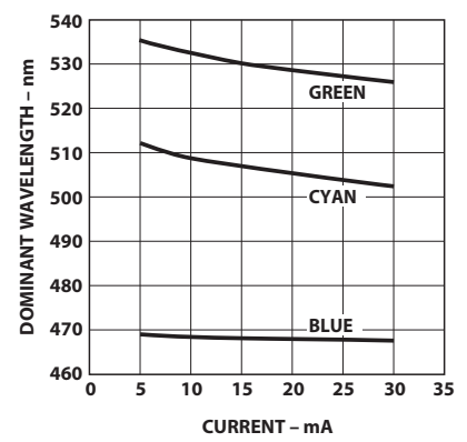
Figure 5. Dominant wavelength vs. forward current – InGaP devices.
