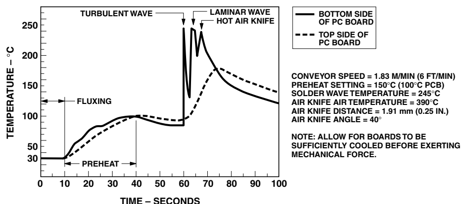
Figure 11. Recommended wave soldering profile.
