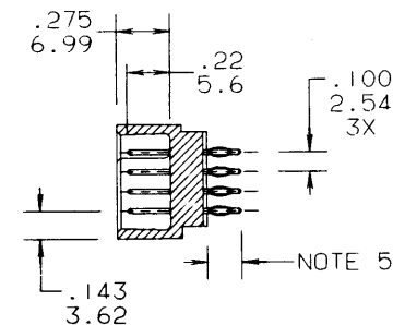
SECTION X-X
