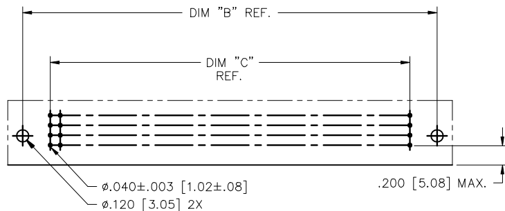
SECTION U-U
