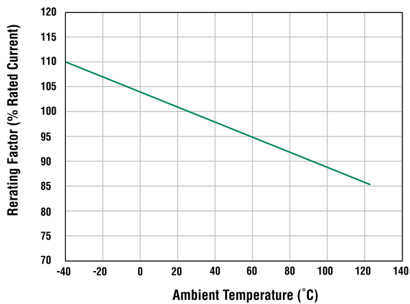
MAXI Fuse Temperature Derating Curve
