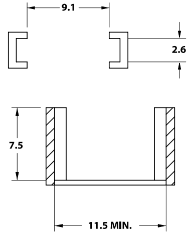
Recommended Mating Cavity
