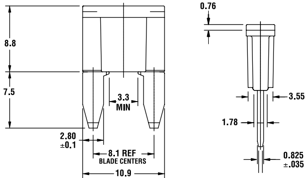
Dimensions in mm / Maße in mm
