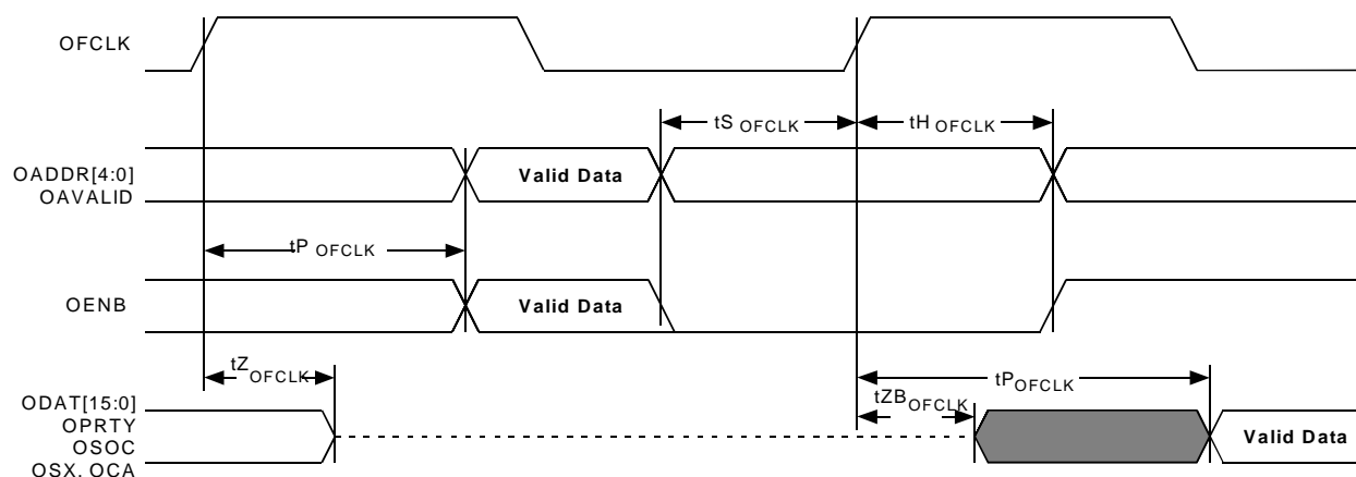
Fig. 27 Egress SCI-PHY/Any-PHY Interface Timing
