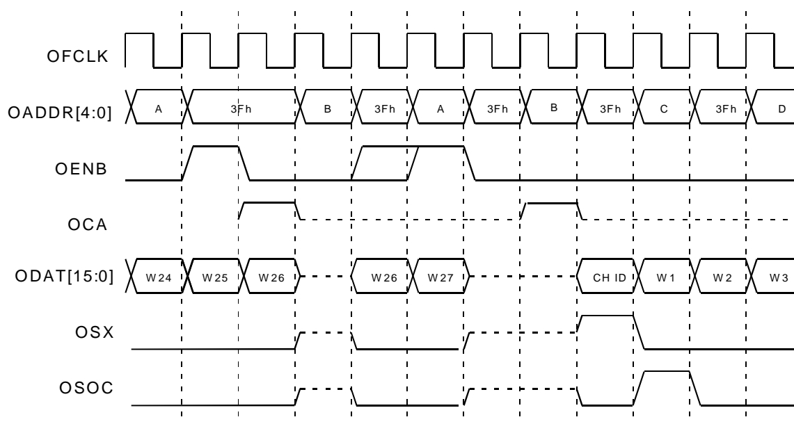
Fig. 19 Any-PHY Interface, Output Bus Slave Transfer Timing
