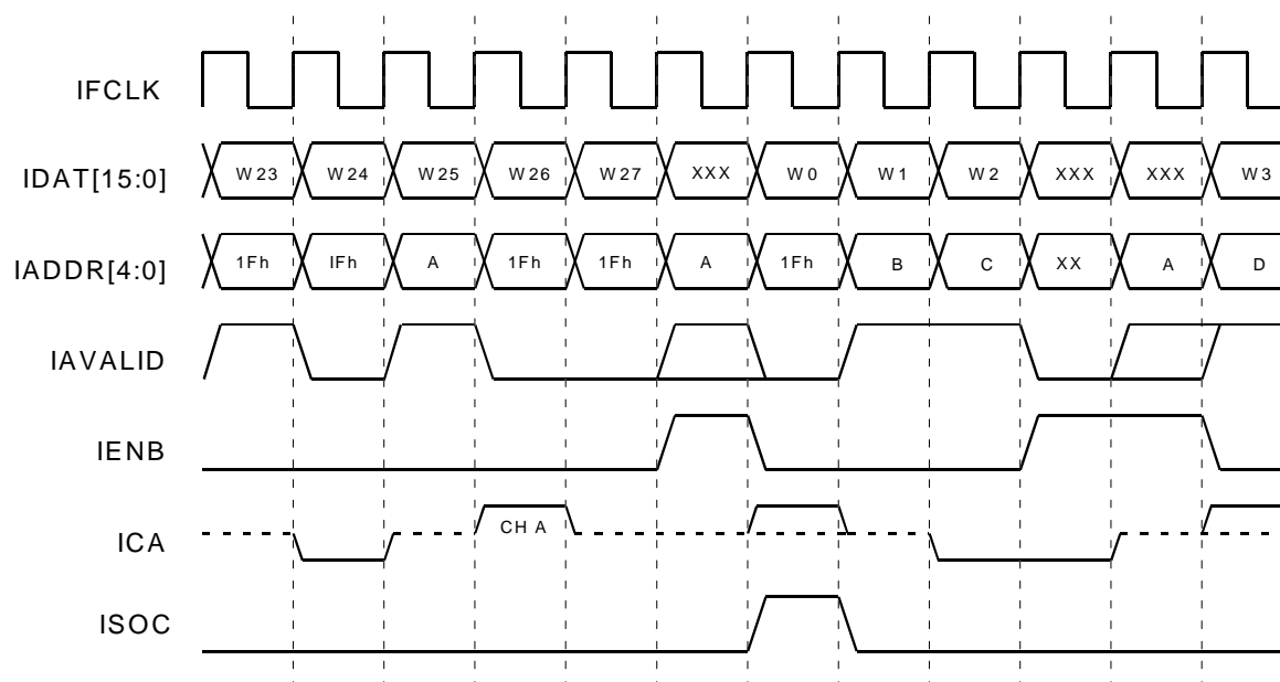
Fig. 14 SCI-PHY Interface, Input Bus Slave Transfer Timing
