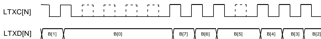
Fig. 20 Clocked Serial Data Transmit Interface
