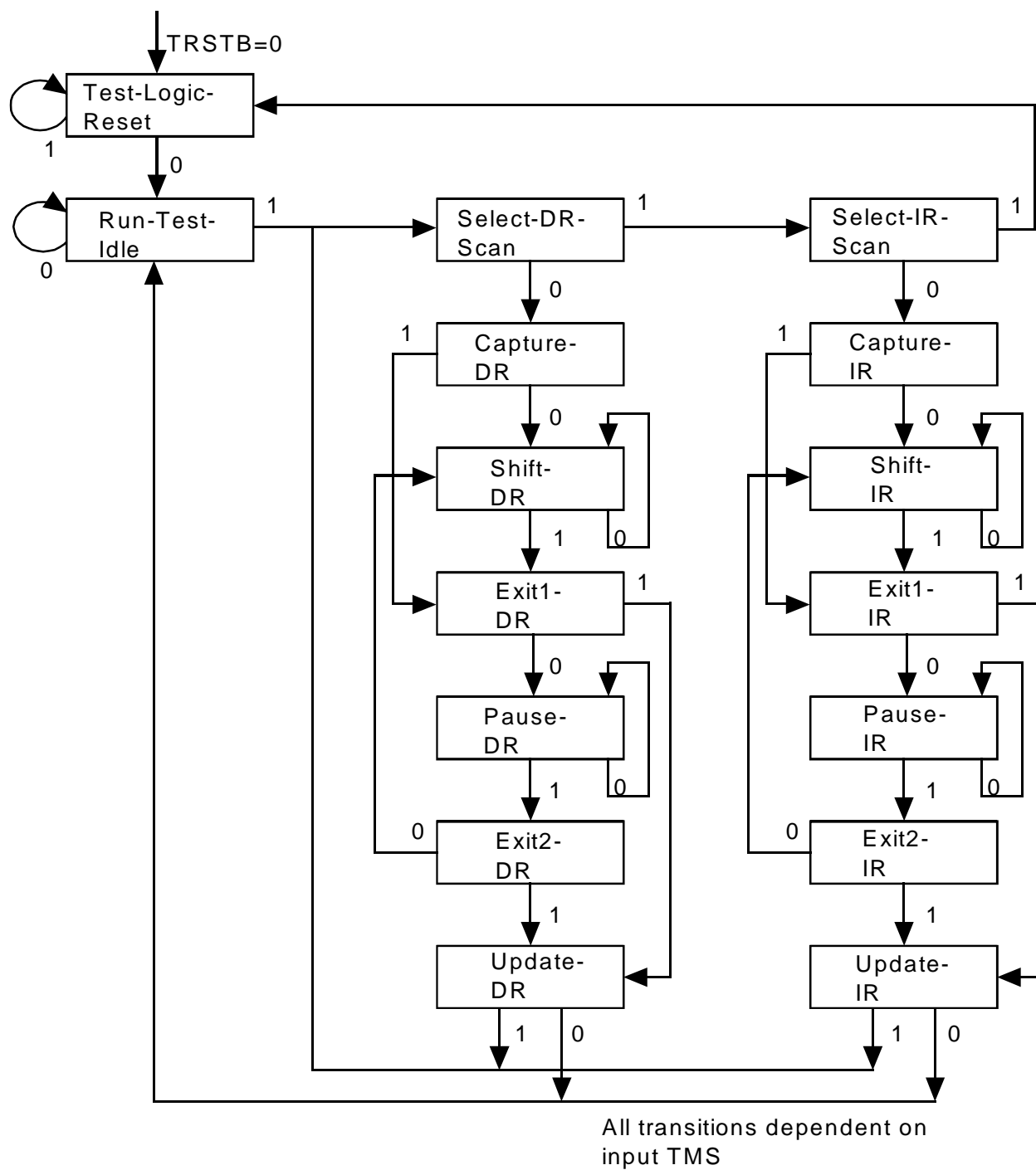
Fig. 13 TAP Controller Finite State Machine
