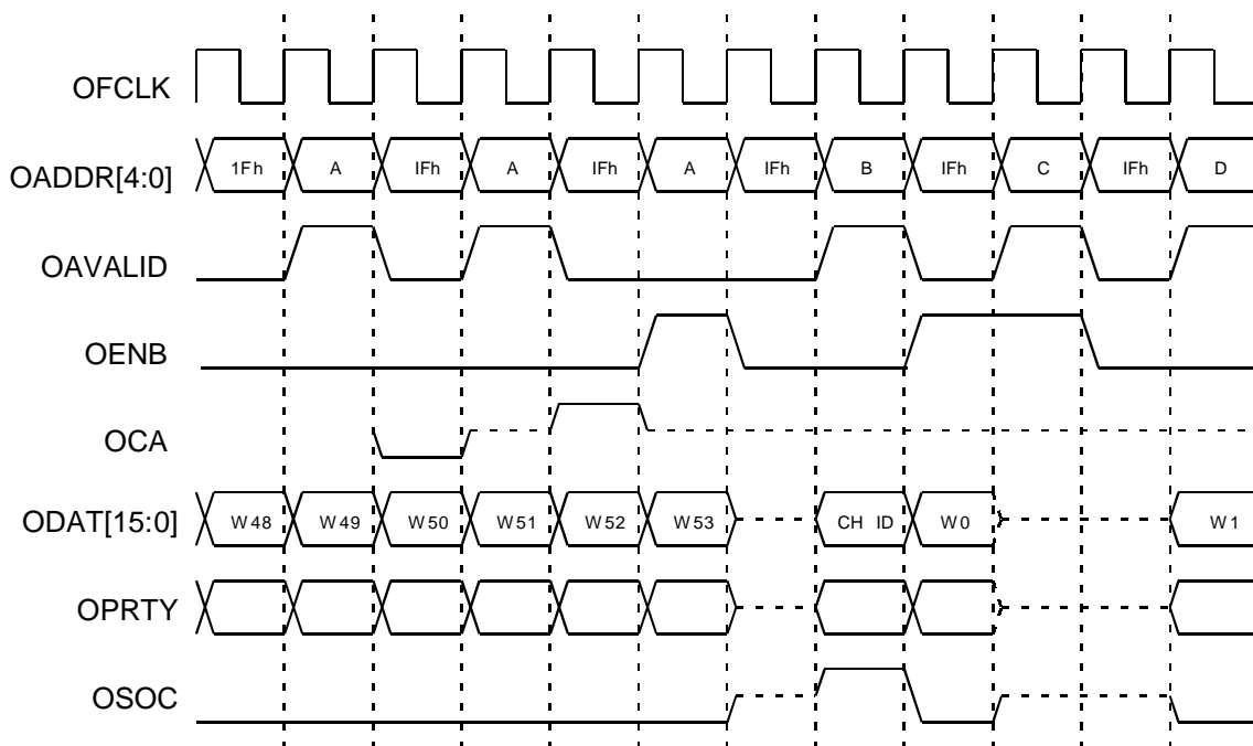
Fig. 17 SCI-PHY Interface, Output Bus Slave Transfer Timing
