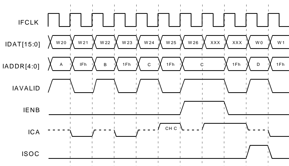
Fig. 15 SCI-PHY Interface, Input Bus Master Transfer Timing
