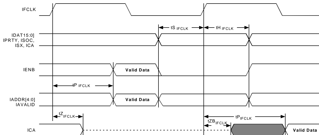
Fig. 26 Ingress SCI-PHY/Any-PHY Interface Timing
