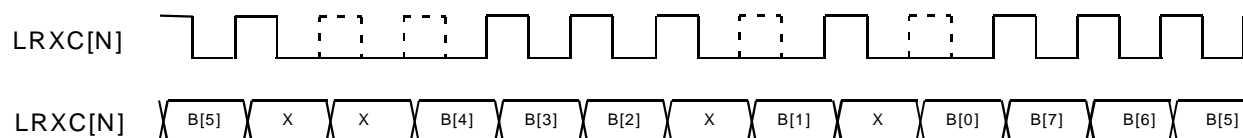
Fig. 22 Clocked Serial Data Receive Interface
