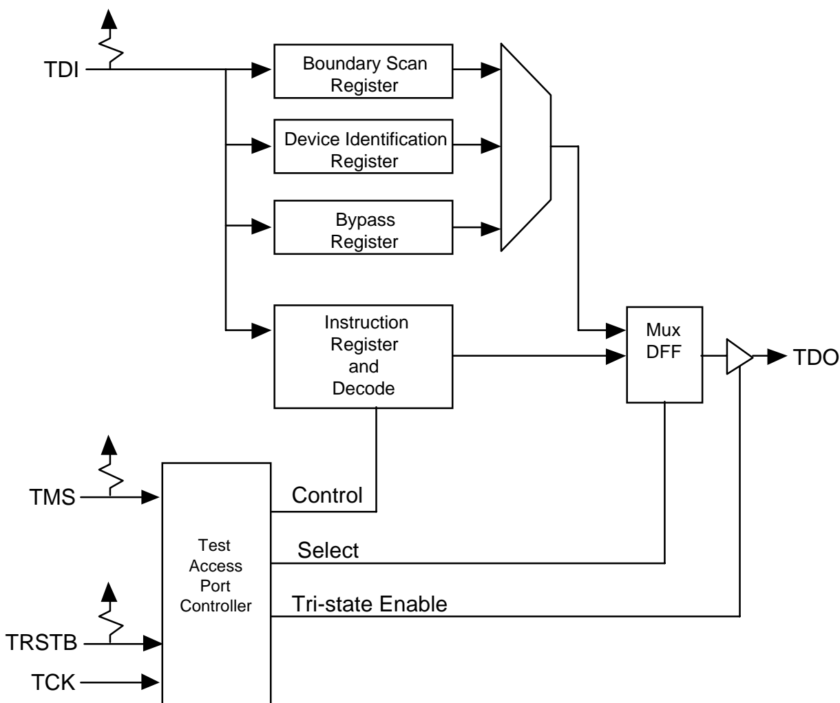
Fig. 12 Boundary Scan Architecture
