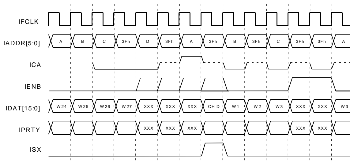
Fig. 16 Any-PHY Interface, Input Bus Slave Transfer Timing
