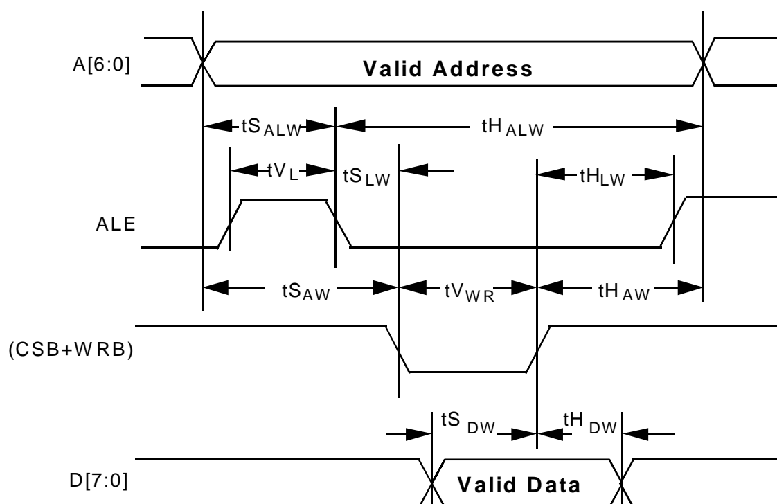
Fig. 24 Microprocessor Interface Write Timing
