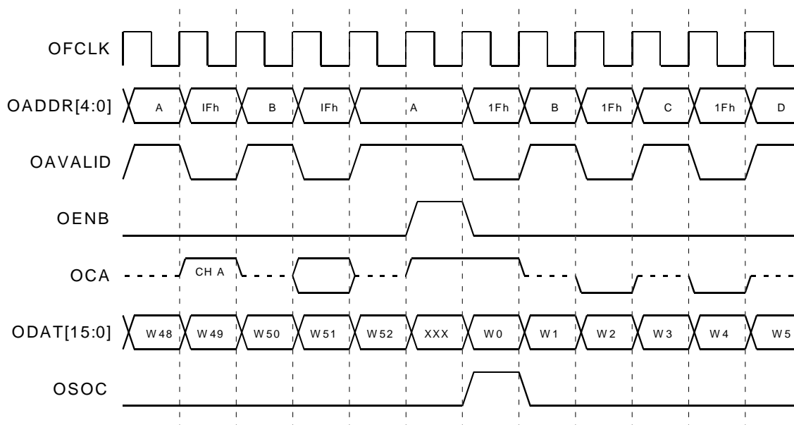
Fig. 18 SCI-PHY Interface, Output Bus Master Transfer Timing
