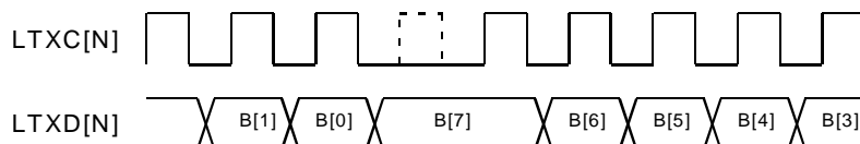
Fig. 21 Clocked Serial Data Transmit Interface, Byte Aligned Data
