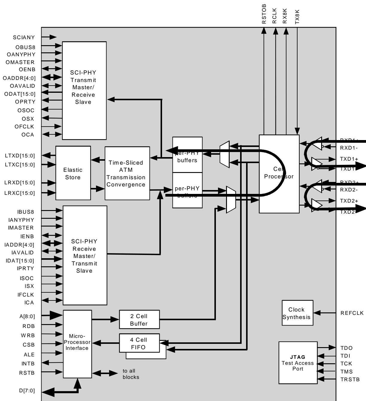
Fig. 10 Datapath Loopback
