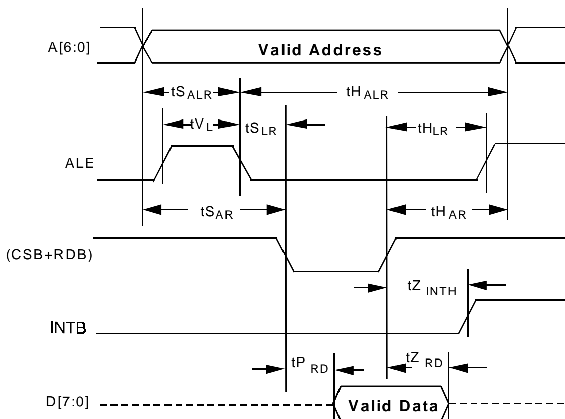
Fig. 23 Microprocessor Interface Read Timing
