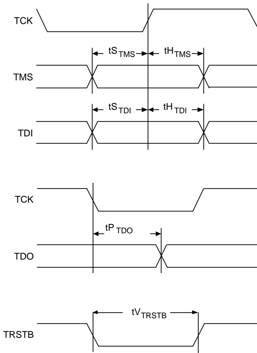
Fig. 28 JTAG Port Interface Timing
