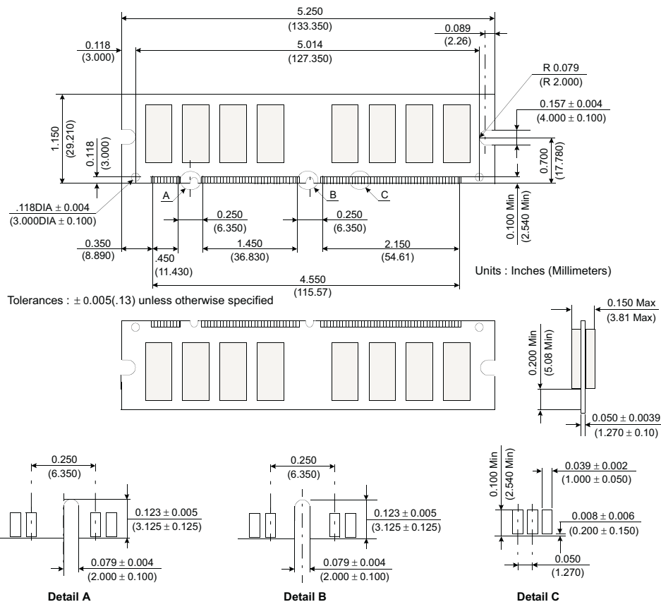
Figure 1: KVR133X64C3L/512 168-Pin SDRAM Module
