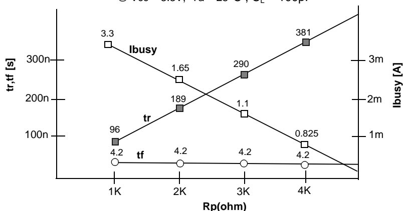
Fig 23 R_p vs t_r, t_f & R_p vs i_{busy}
