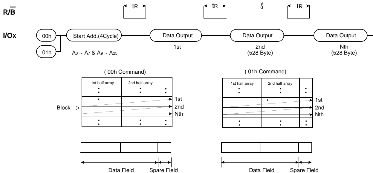
Figure 9. Sequential Row Read1 Operation (only for K9F1208U0A-Y and K9F1208U0A-V, valid within a block)
