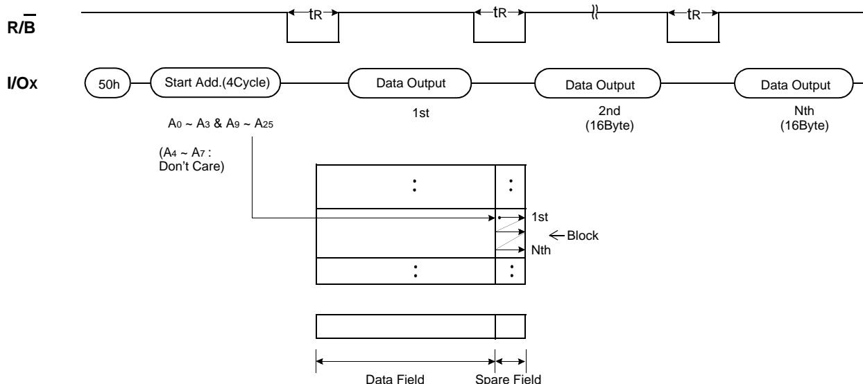
Figure 10. Sequential Row Read2 Operation (only for K9F1208U0A-Y and K9F1208U0A-V, valid within a block )
