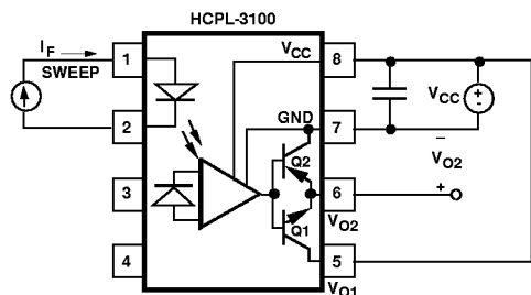
Figure 8. Test Circuit for Threshold Input Current I_{FLIH} .
