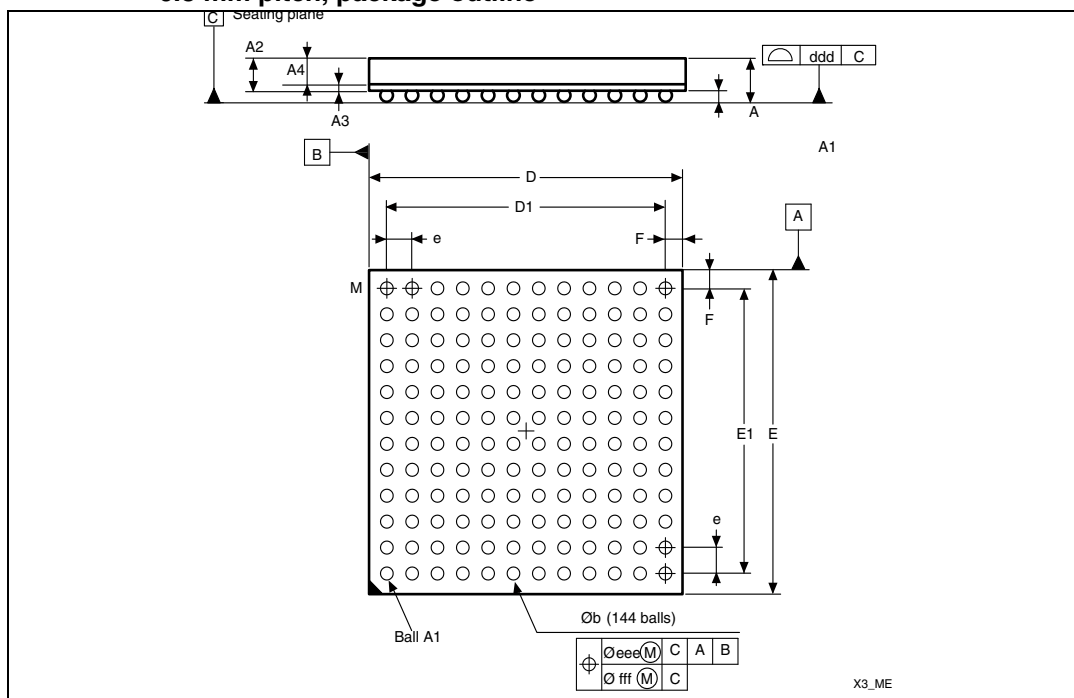
Figure 58. LFBGA144 – 144-ball low profile fine pitch ball grid array, 10 x 10 mm, 0.8 mm pitch, package outline
