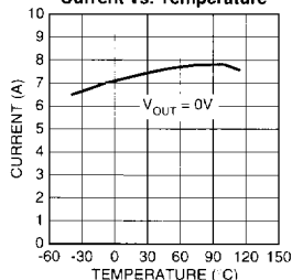
MIC2950x-5.0 Short Circuit Current vs. Temperature
