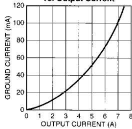
MIC2975x Ground Current vs. Output Current
