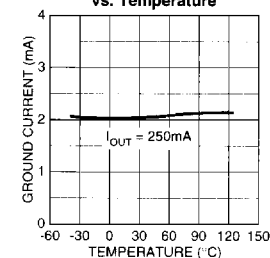
MIC2975x Ground Current vs. Temperature
