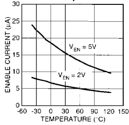
MIC29501-xx/2 Enable Current vs. Temperature
