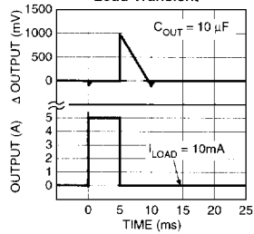
MIC2950x Load Transient
