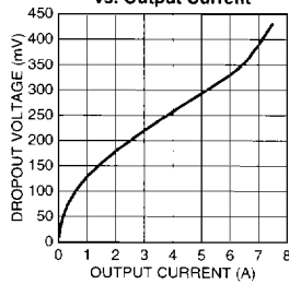
MIC2975x Dropout Voltage vs. Output Current
