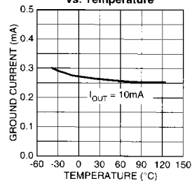
MIC2975x Ground Current vs. Temperature
