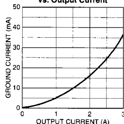
MIC2930x Ground Current vs. Output Current
