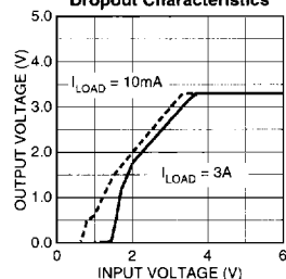
MIC29300-3.3 Dropout Characteristics
