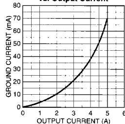
MIC2950x Ground Current vs. Output Current
