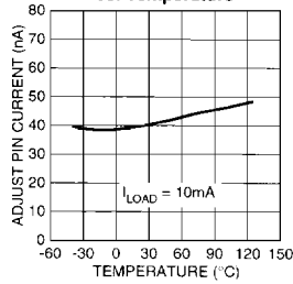
MIC29502/3 Adjust Pin Current vs. Temperature
