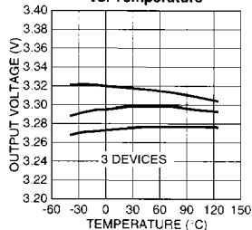
MIC29500-3.3 Output Voltage vs. Temperature
