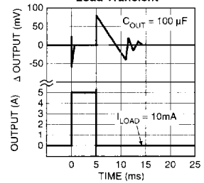
MIC2950x Load Transient
