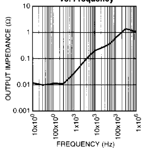
MIC2915x Output Impedance vs. Frequency
