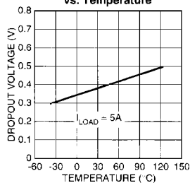
MIC2950x Dropout Voltage vs. Temperature
