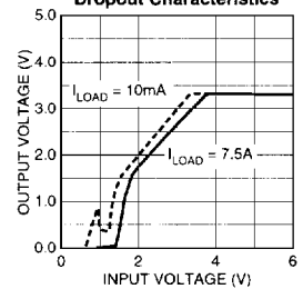
MIC29750-3.3 Dropout Characteristics
