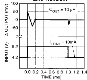
MIC2950x Line Transient
