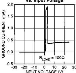
MIC2930x Ground Current vs. Input Voltage
