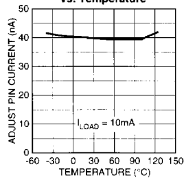
MIC29152/3 Adjust Pin Current vs. Temperature
