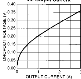
MIC2930x Dropout Voltage vs. Output Current
