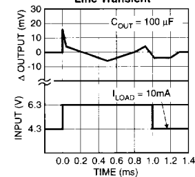
MIC2975x Line Transient
