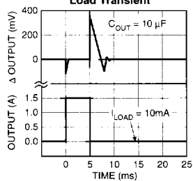
MIC2915x Load Transient
