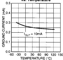
MIC2930x Ground Current vs. Temperature
