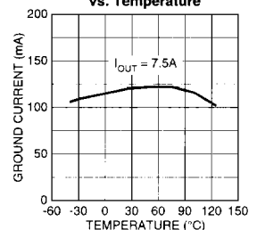
MIC2975x Ground Current vs. Temperature
