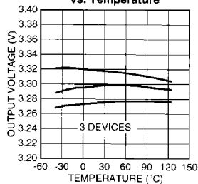
MIC29750-3.3 Output Voltage vs. Temperature
