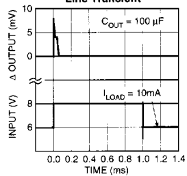
MIC2915x Line Transient
