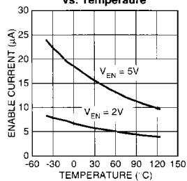
MIC29151-xx/2 Enable Current vs. Temperature
