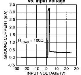
MIC2975x Ground Current vs. Input Voltage
