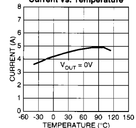
MIC29300-5.0 Short Circuit Current vs. Temperature
