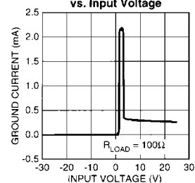
MIC2950x Ground Current vs. Input Voltage
