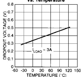
MIC2930x Dropout Voltage vs. Temperature
