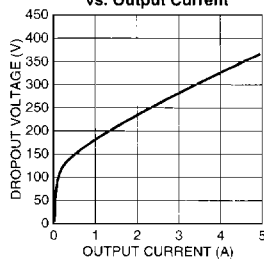
MIC2950x Dropout Voltage vs. Output Current
