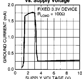
MIC2930x Ground Current vs. Supply Voltage
