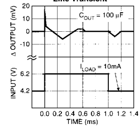
MIC2950x Line Transient
