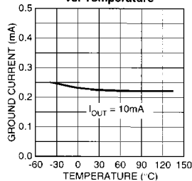
MIC2950x Ground Current vs. Temperature
