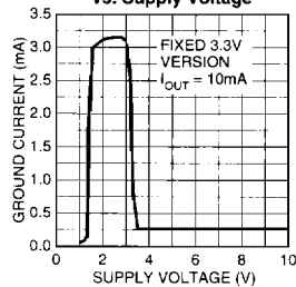
MIC2975x Ground Current vs. Supply Voltage
