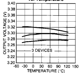
MIC29300-3.3 Output Voltage vs. Temperature
