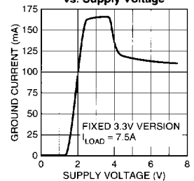
MIC2975x Ground Current vs. Supply Voltage
