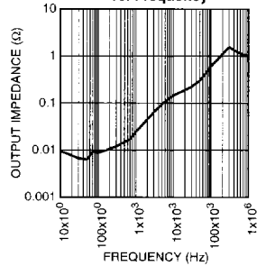
MIC2950x Output Impedance vs. Frequency
