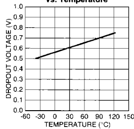
MIC2975x Dropout Voltage vs. Temperature
