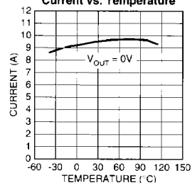
MIC29750-5.0 Short Circuit Current vs. Temperature
