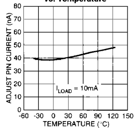
MIC29752/3 Adjust Pin Current vs. Temperature
