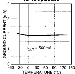
MIC2950x Ground Current vs. Temperature
