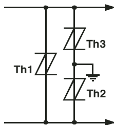
Figure 17. MULTI-POINT PROTECTION
