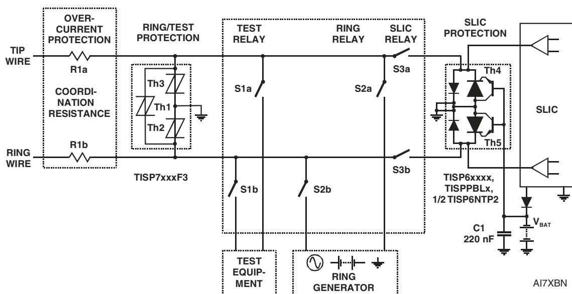
Figure 23. Line Card Ring/Test Protection
