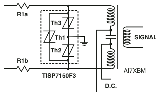
Figure 22. ISDN Protection
