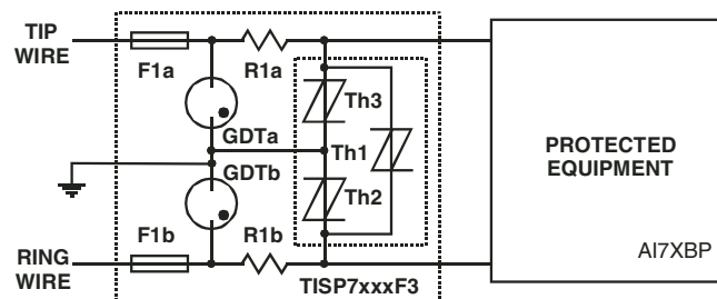
Figure 21. Protection Module
