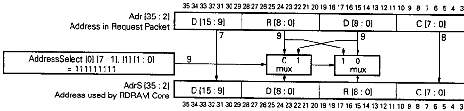
Figure 9-1. AddressMapping Hardware
