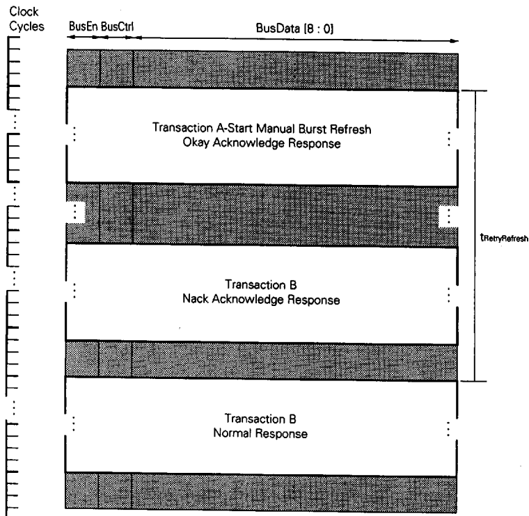
Figure 8-2. Transaction Holdoff Due to Burst Refresh
