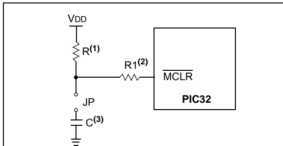
FIGURE 2-2: MCLR PIN CONNECTIONS
