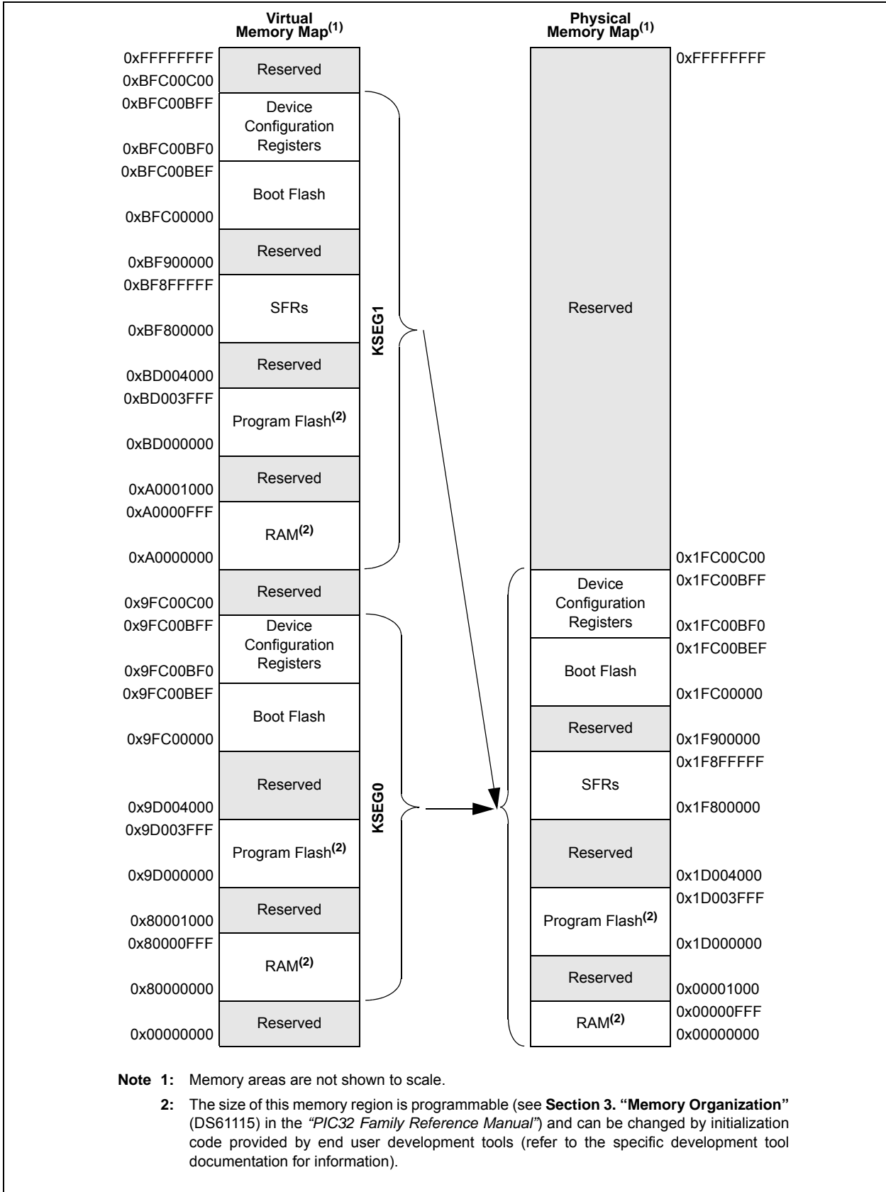
FIGURE 4-1: MEMORY MAP ON RESET FOR PIC32MX11X/21X DEVICES
