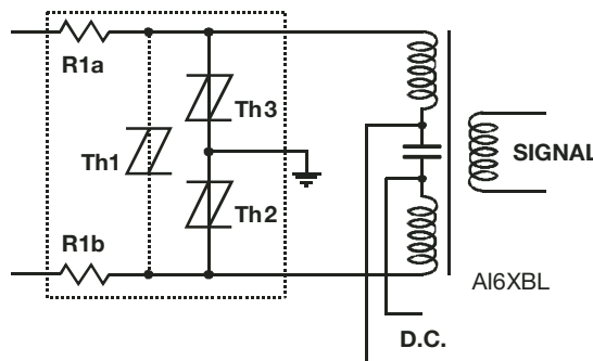
Figure 17. ISDN Protection
