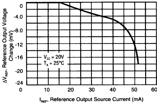
REFERENCE OUTPUT VOLTAGE CHANGE versus OUTPUT SOURCE CURRENT
