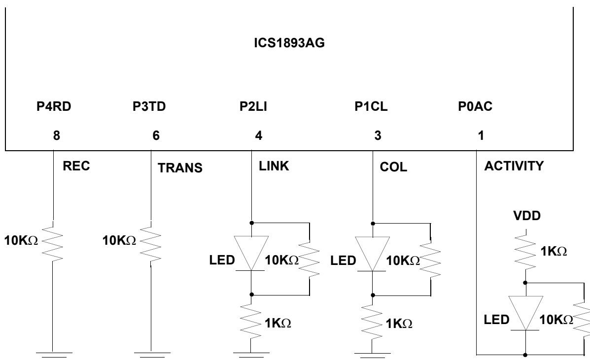
Figure 6-4. ICS1893AG LED - PHY Interface
