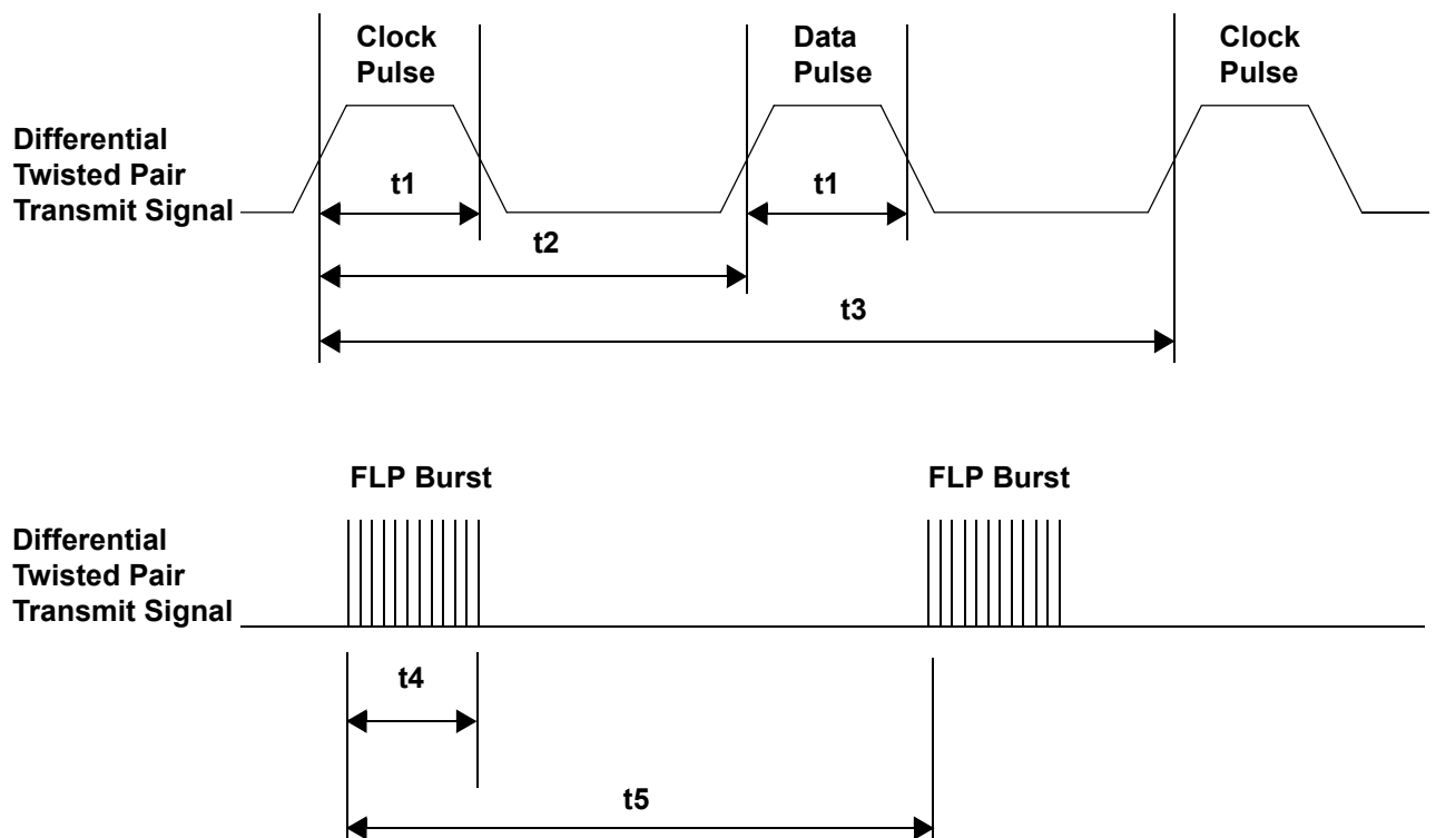
Figure 10-21. Auto-Negotiation Fast Link Pulse Timing Diagram
