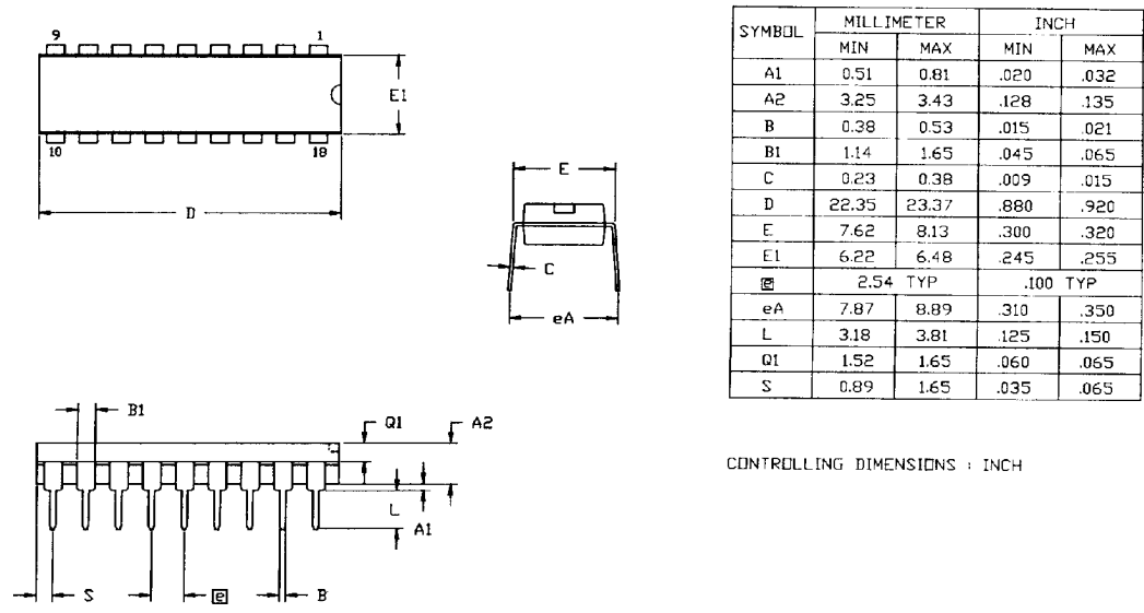
Figure 45. 18-Pin DIP Package Diagram
