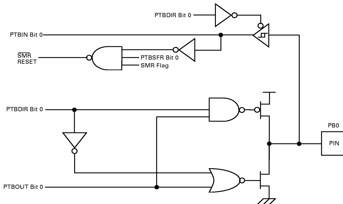
Figure 33. Port B Pin 0 Diagram
