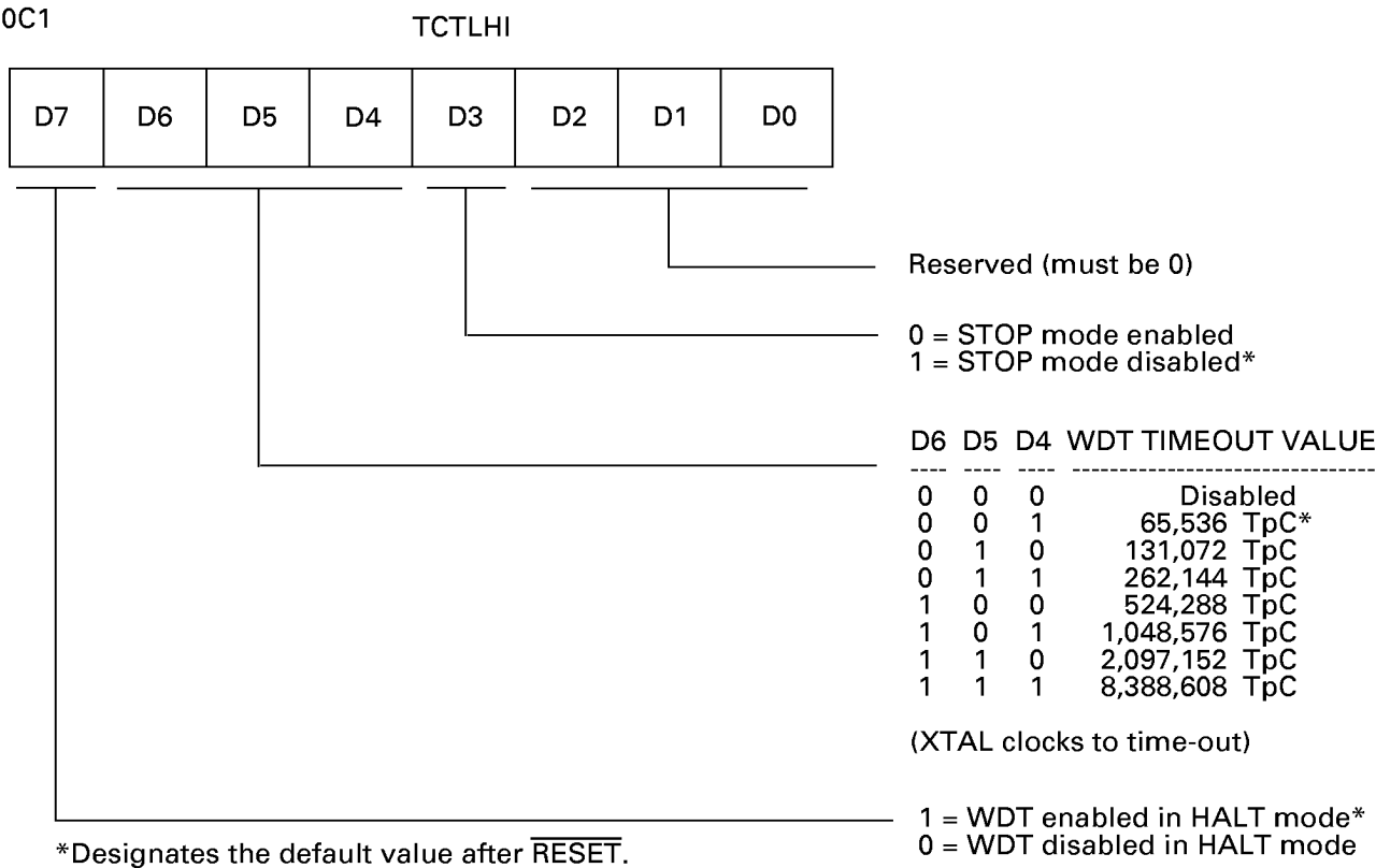
Figure 11. TCTLHI Register for Control of WDT
