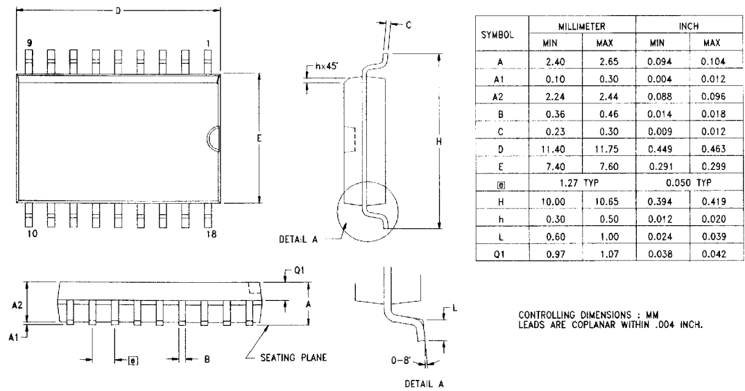
Figure 46. 18-Pin SOIC Package Diagram
