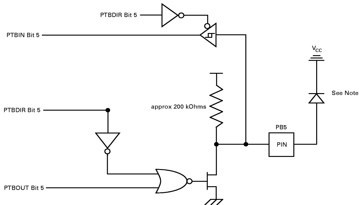
Figure 34. Port B Pin 5 Diagram
