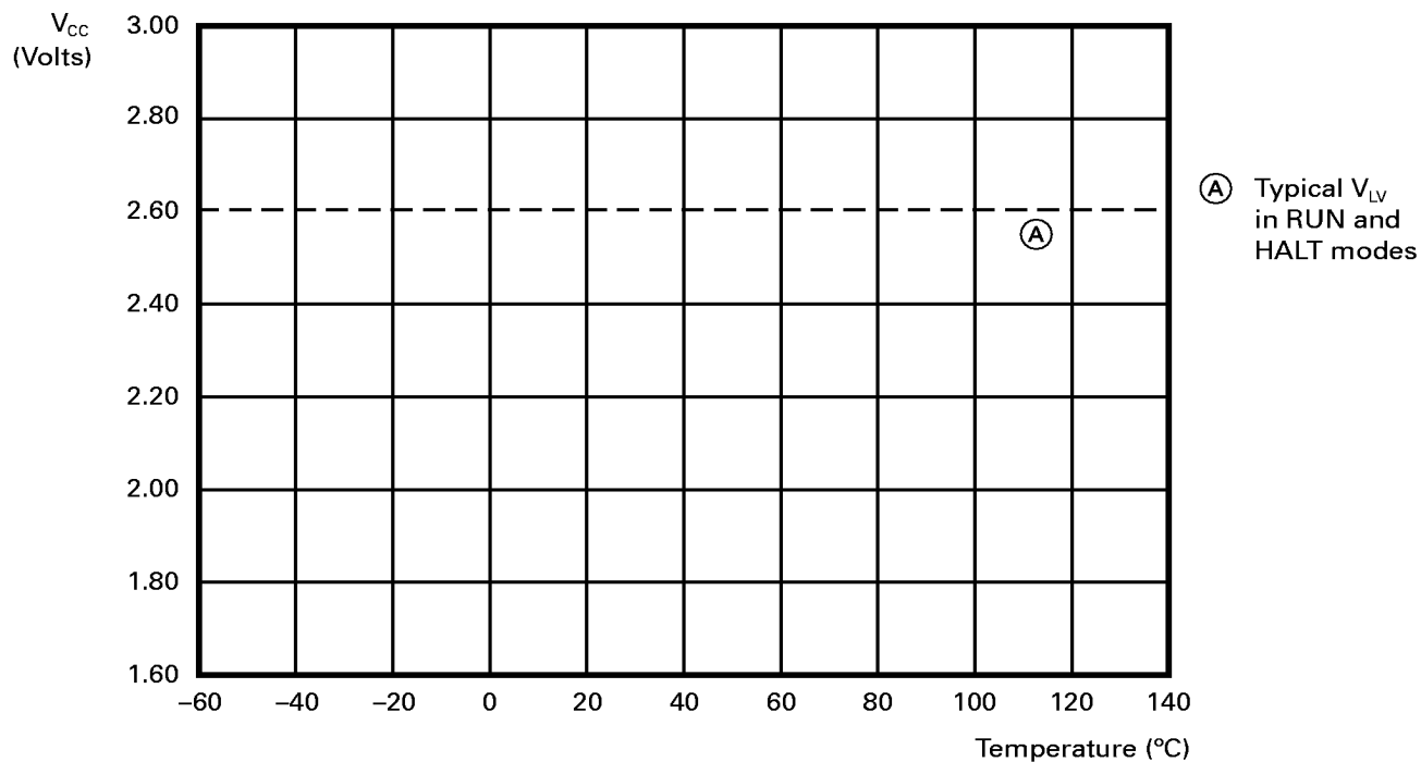
Figure 42. Typical Low Voltage Protection vs. Temperature
