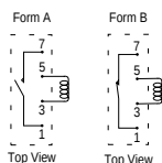
SIL4/DSS4 Pinout
