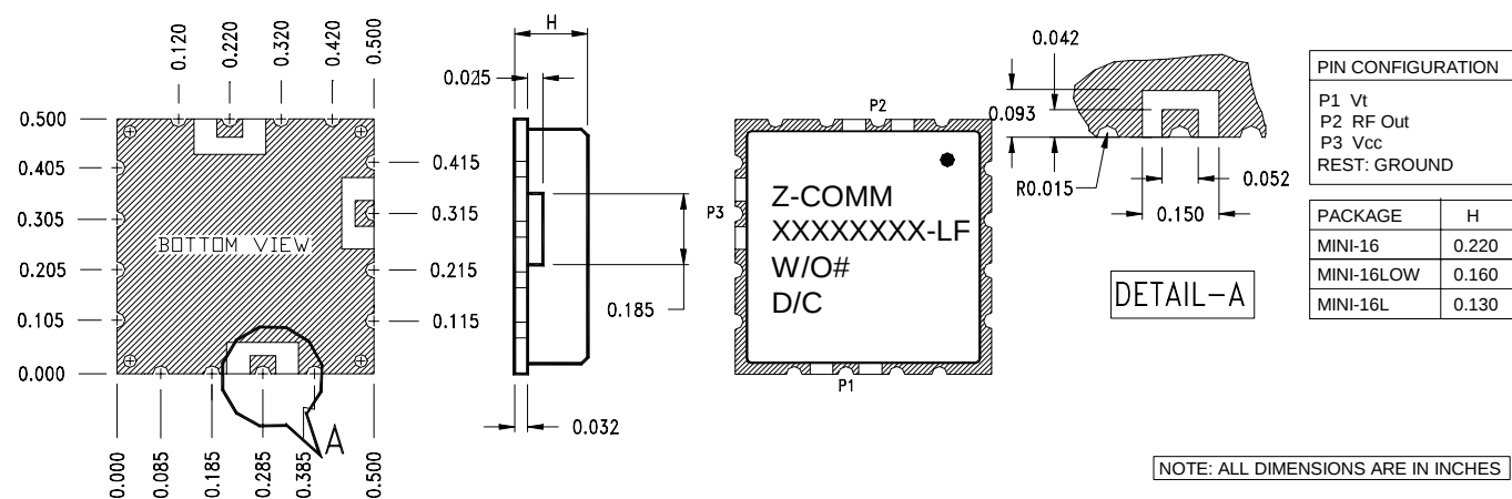
PHYSICAL DIMENSIONS
