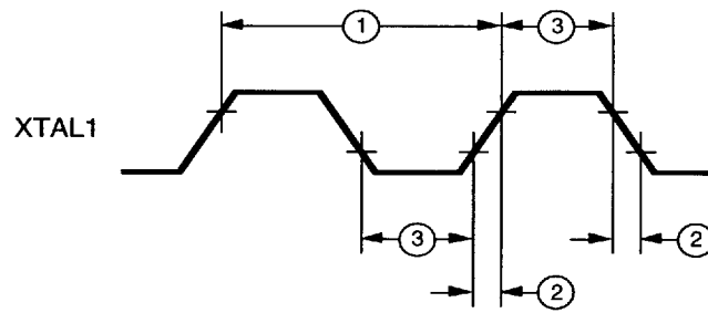
External Clock
