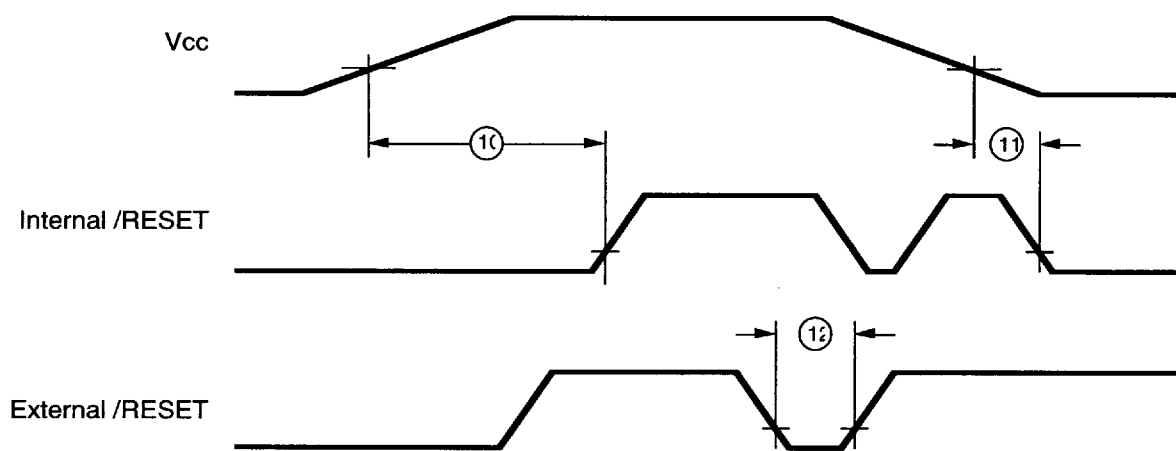
Power-On Reset
