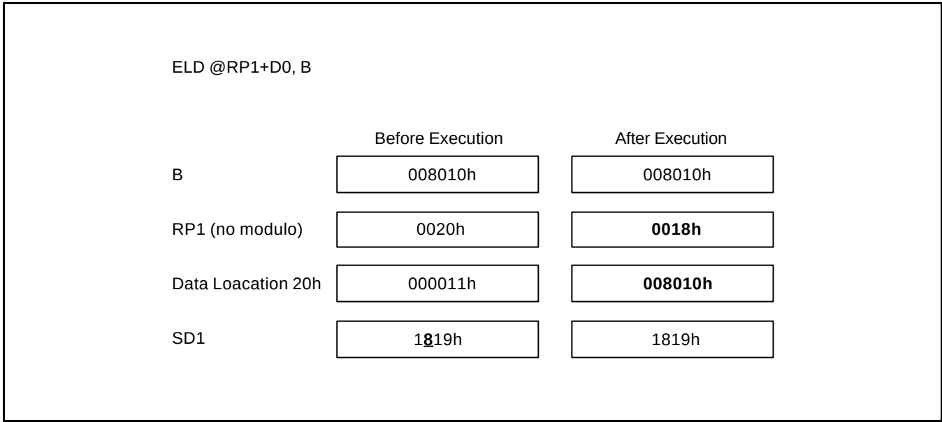
Figure 25-19. Indirect Addressing Example II (Write Operation)
