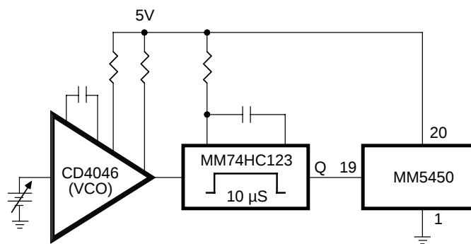
Figure 11. Brightness Control Varying the Duty Cycle
