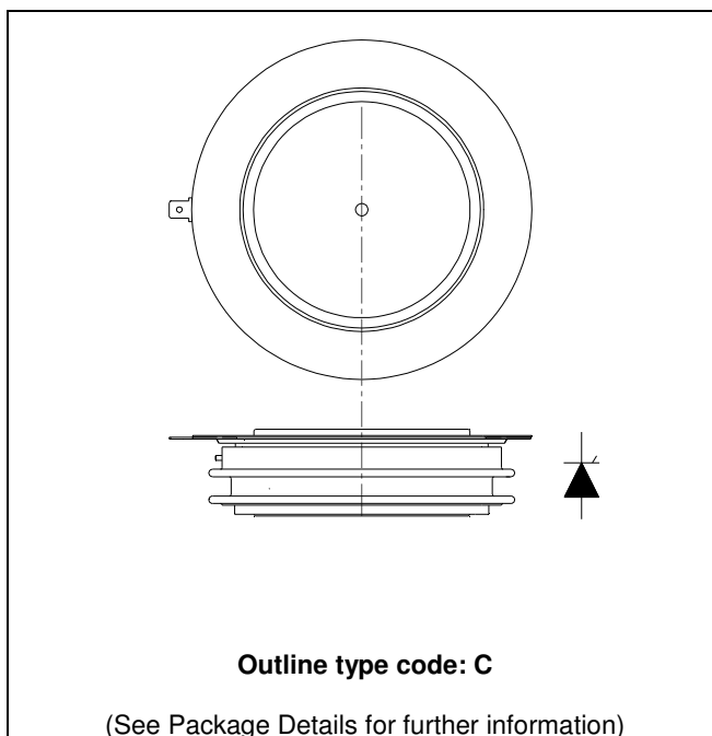
Fig. 1 Package outline
