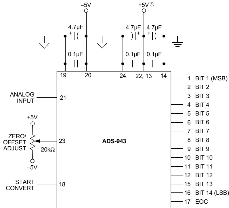
Figure 3. Connection Diagram
