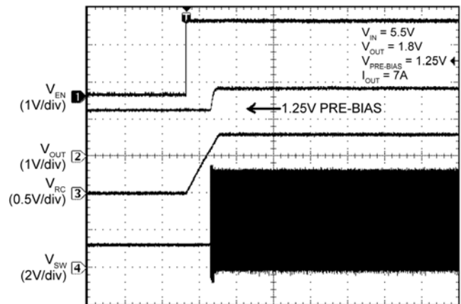
Time (1ms/div)
