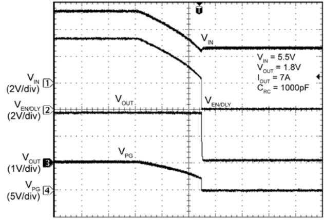
Time (2ms/div)
