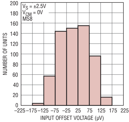
V_{OS} Distribution
