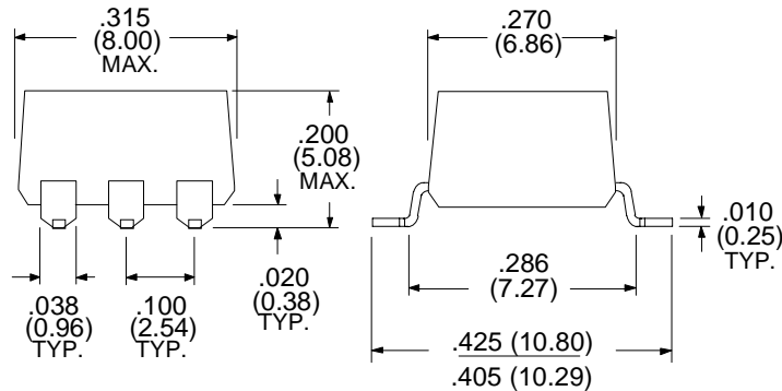
Physical Dimensions inches (mm)
