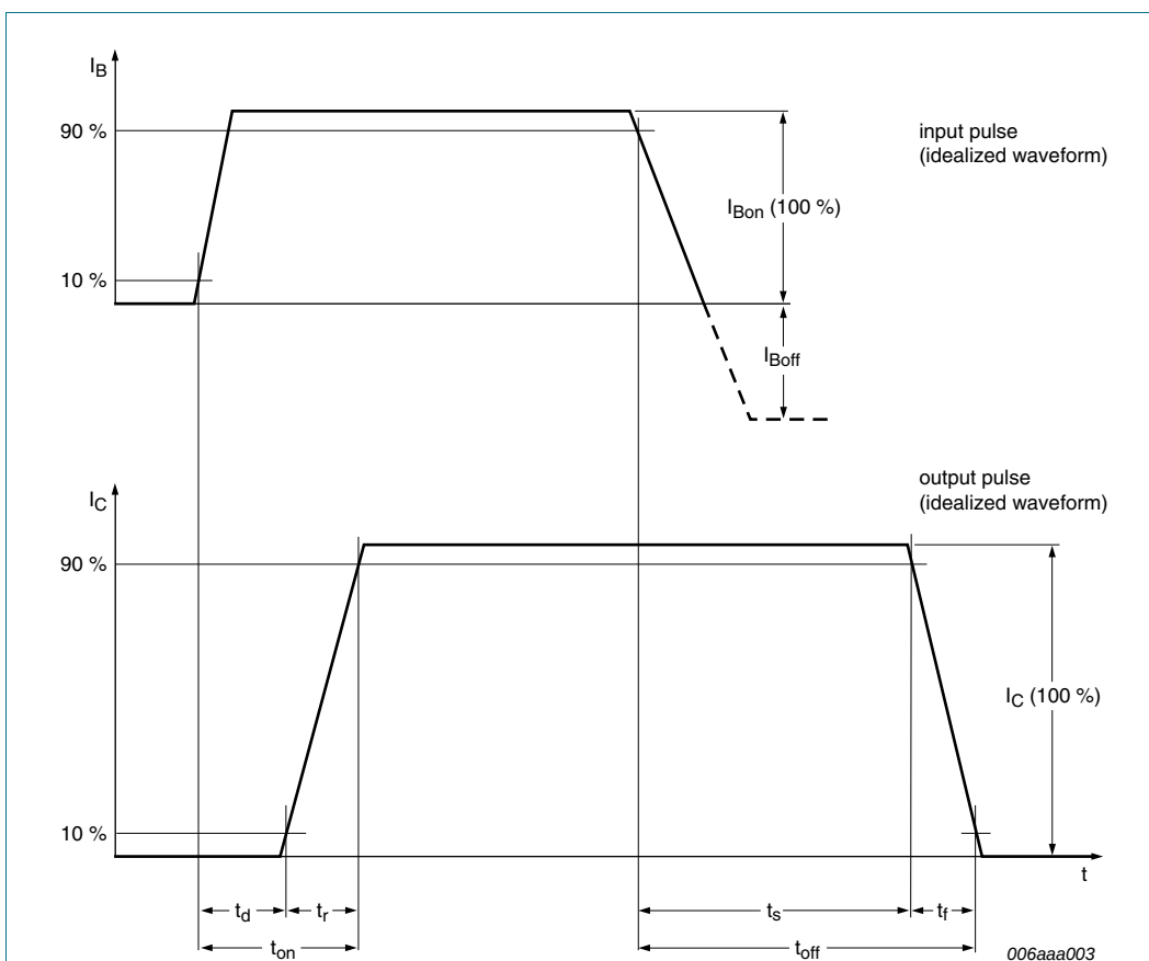
Fig 14. BISS transistor switching time definition
