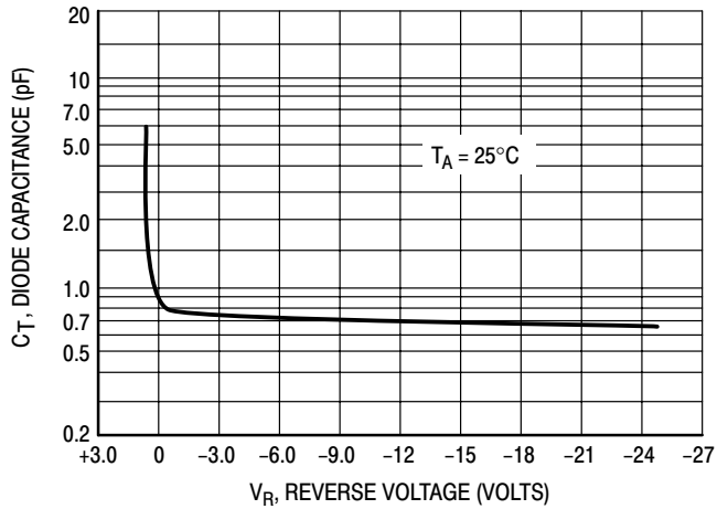
Figure 3. Diode Capacitance
