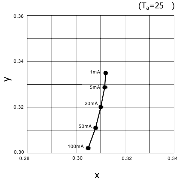
(6) forward current vs. chromaticity diagram
