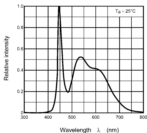
Fig. 8.4 Wavelength characteristic
