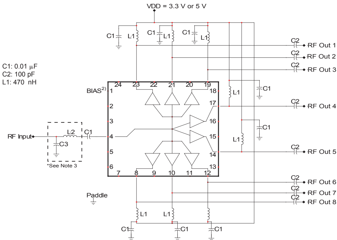
Figure 3: 8-Way Active Splitter Digital Application Circuit
