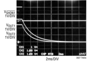
Turn-Off Waveforms
