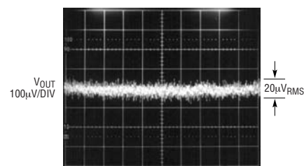
10Hz to 100kHz Output Noise
