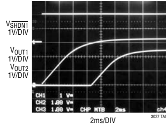
Turn-On Waveforms
