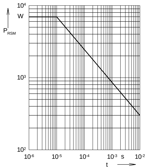
Fig. 3: Power loss
