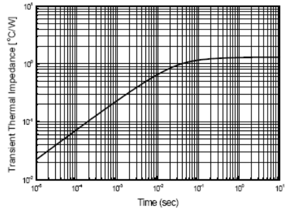
Fig.4 Thermal Response
