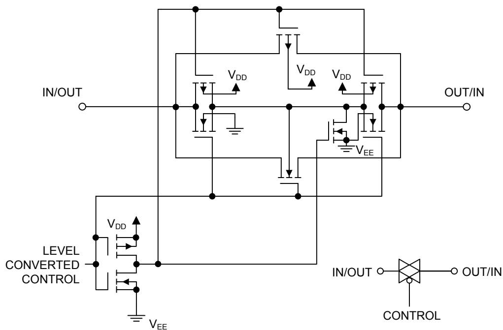
Switch Circuit Schematic
