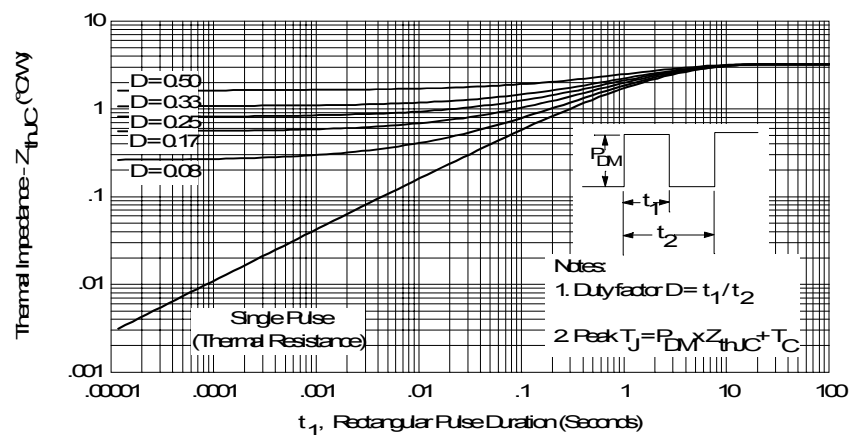
Fig. 4 - Max. Thermal Impedance Z_{thC} Characteristics (Per Leg)
