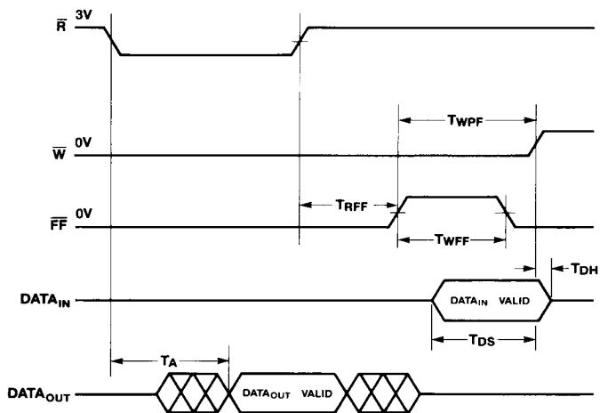
Figure 14. Write Data Flow-Through Mode
