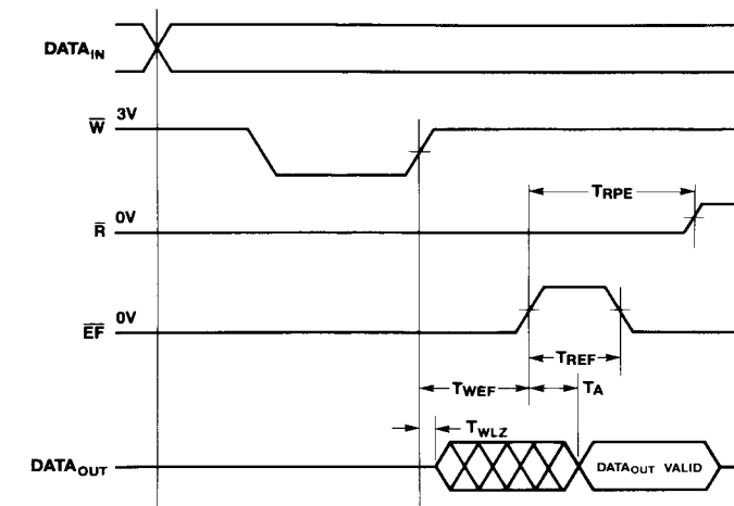
Figure 13. Read Data Flow-Through Mode
